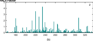
Mass Spectra of each RHALS Factor
